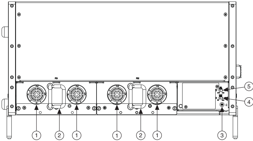
Figure 1-2. Rear View of the PXIe-1066DC Chassis
