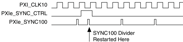
Figure 1-7. PXle_SYNC100 at 3.33 MHz Using PXle_SYNC_CTRL as Restart
