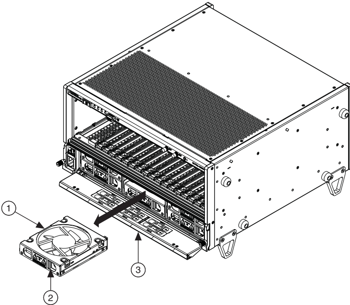
Figure 3-3. PXIe-1066DC Chassis with Fan Assembly Removed
