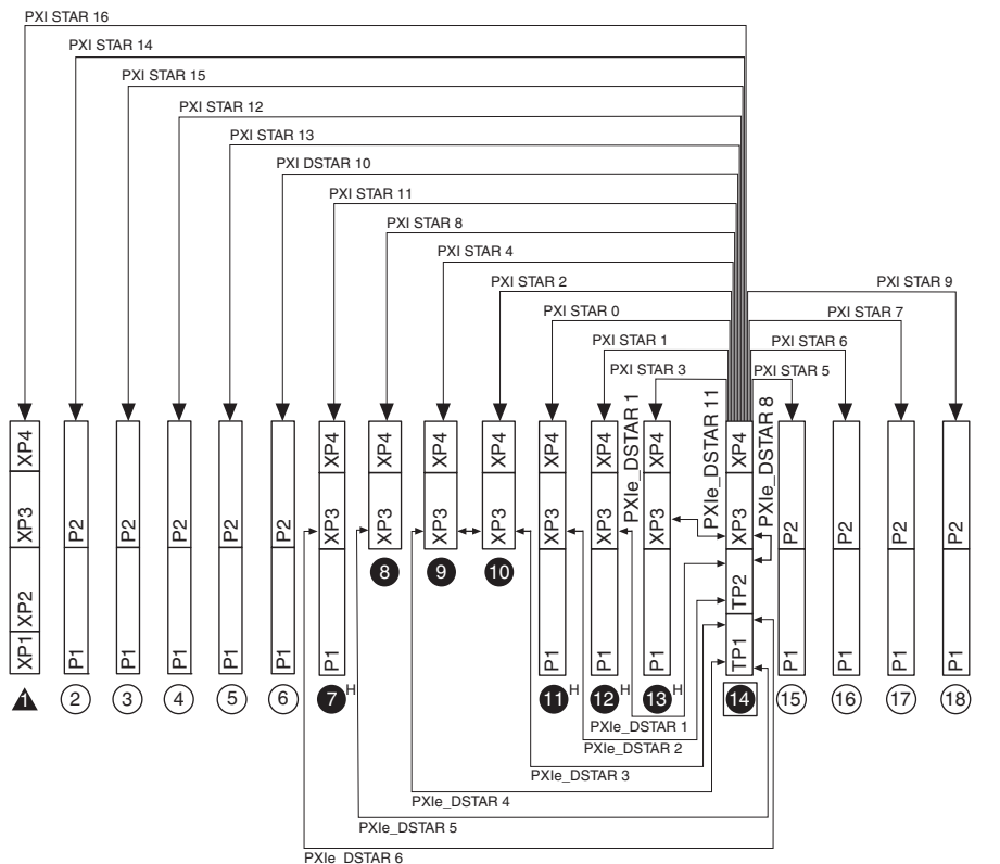
Figure 1-3. PXIe_DSTAR and PXI Star Connectivity Diagram
