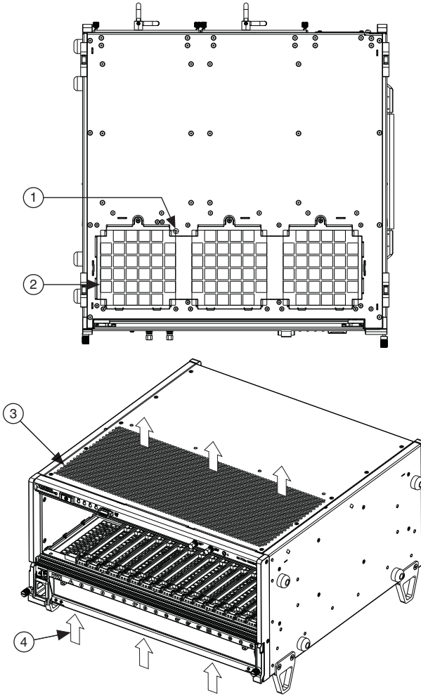
Figure 2-2. PXIe-1066DC Vents
